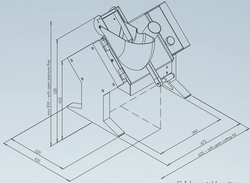
G 5.1 vegetable cutter (Representation)
